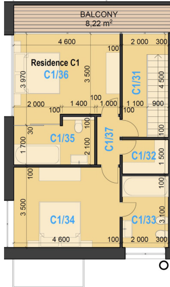
3 RD FLOOR
