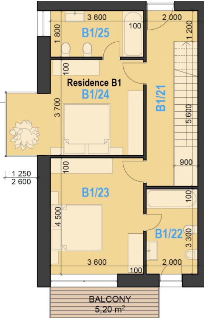
2 ND FLOOR
