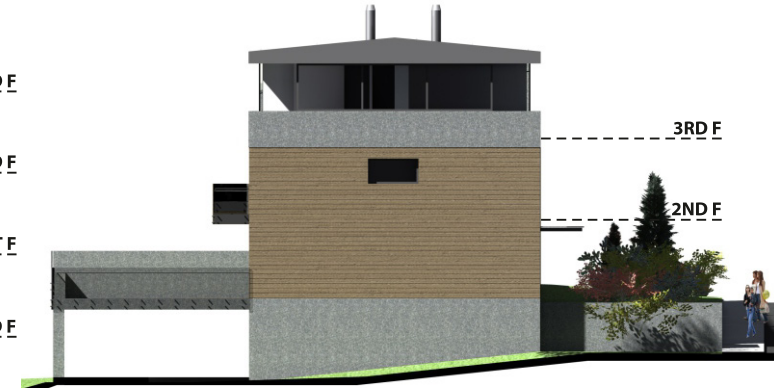
EASTERN VIEW
