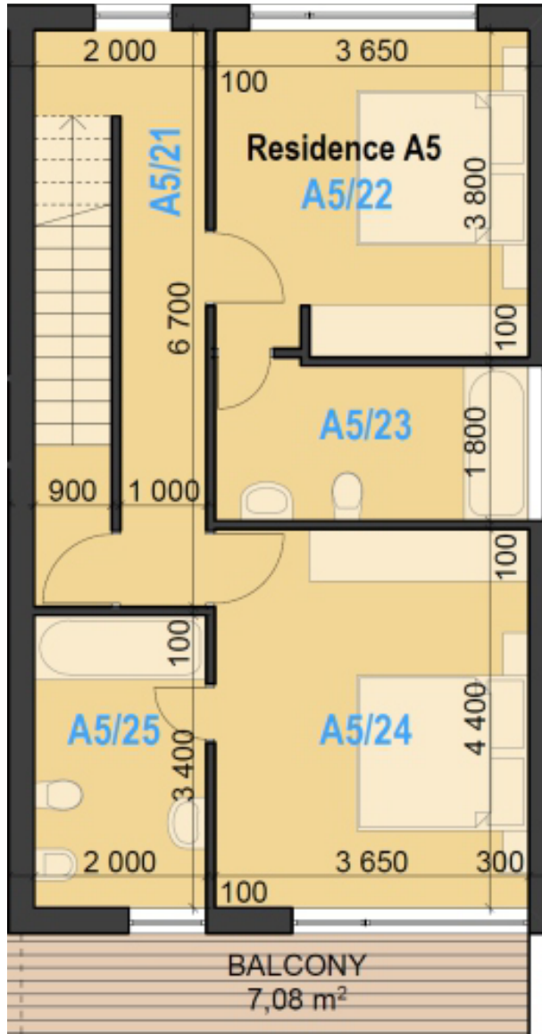
2 ND FLOOR
